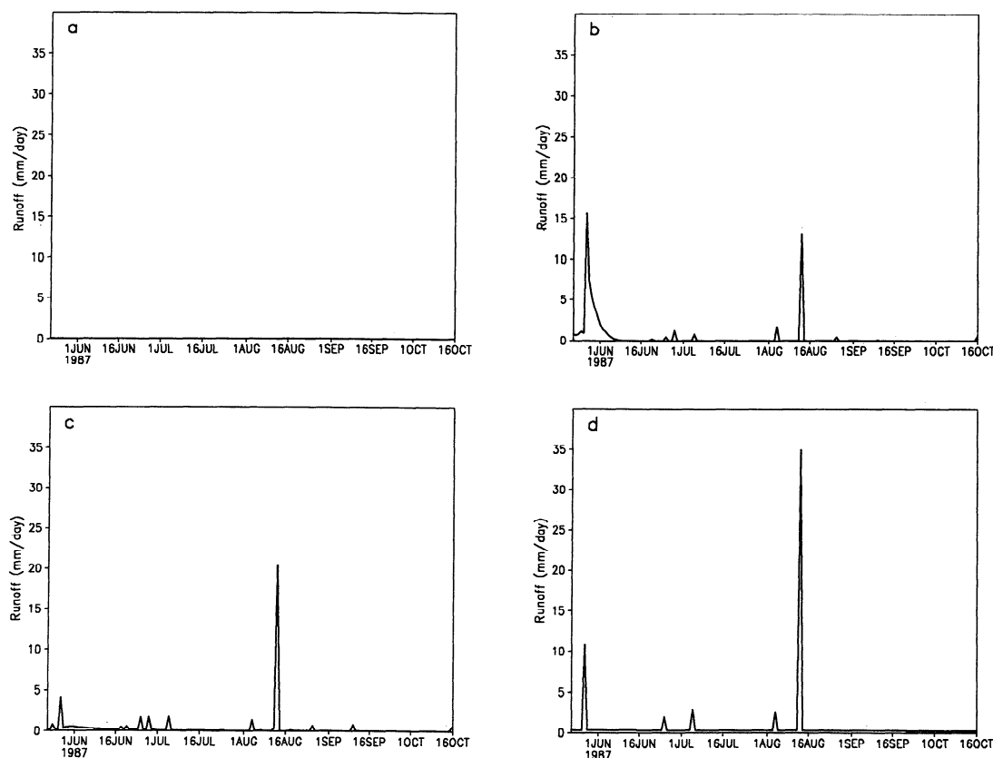
Figure 9. The daily total runoff (in millimeters per day) simulated by four surface models: (a) bucket, (b) SWB, (c) OSU, and (d) SSiB.
