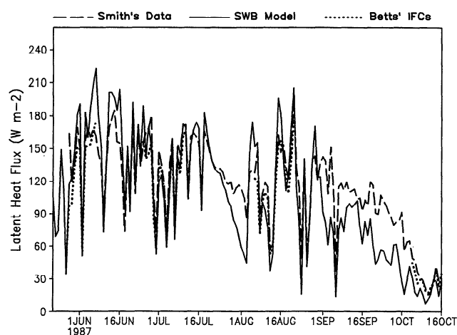
Figure 15. Comparison of daily averaged latent heat fluxes (in watts per square meter) between simulations by the SWB model with a more complex canopy resistance and observations from May 22 to October 16 (compare to Figure 5b).
