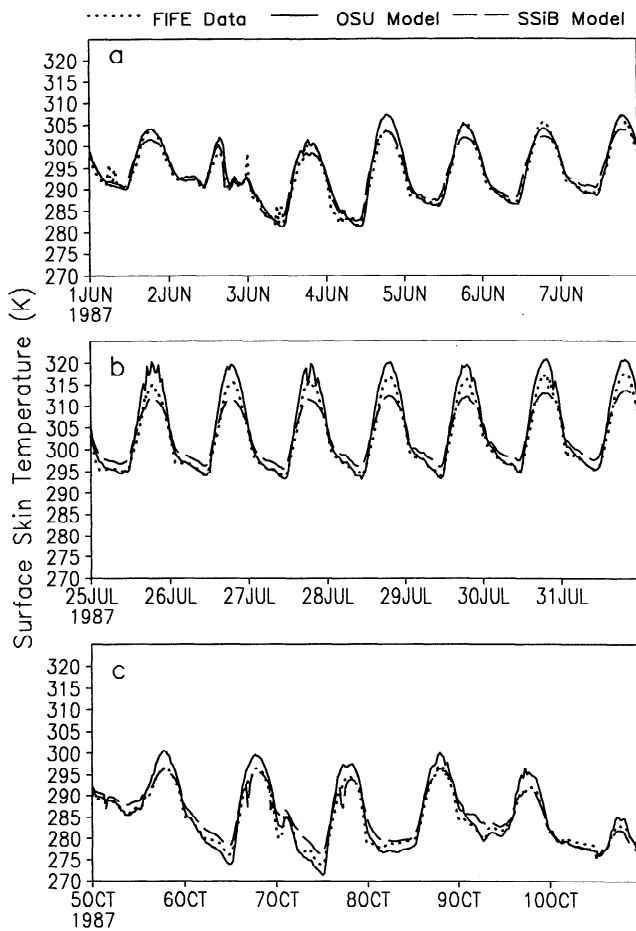
Figure 13. Comparison of diurnal variation of surface skin temperature between the OSU and SSiB model simulations and FIFE observations: (a) June 1–7, (b) July 25–31, and (c) October 5–10.
