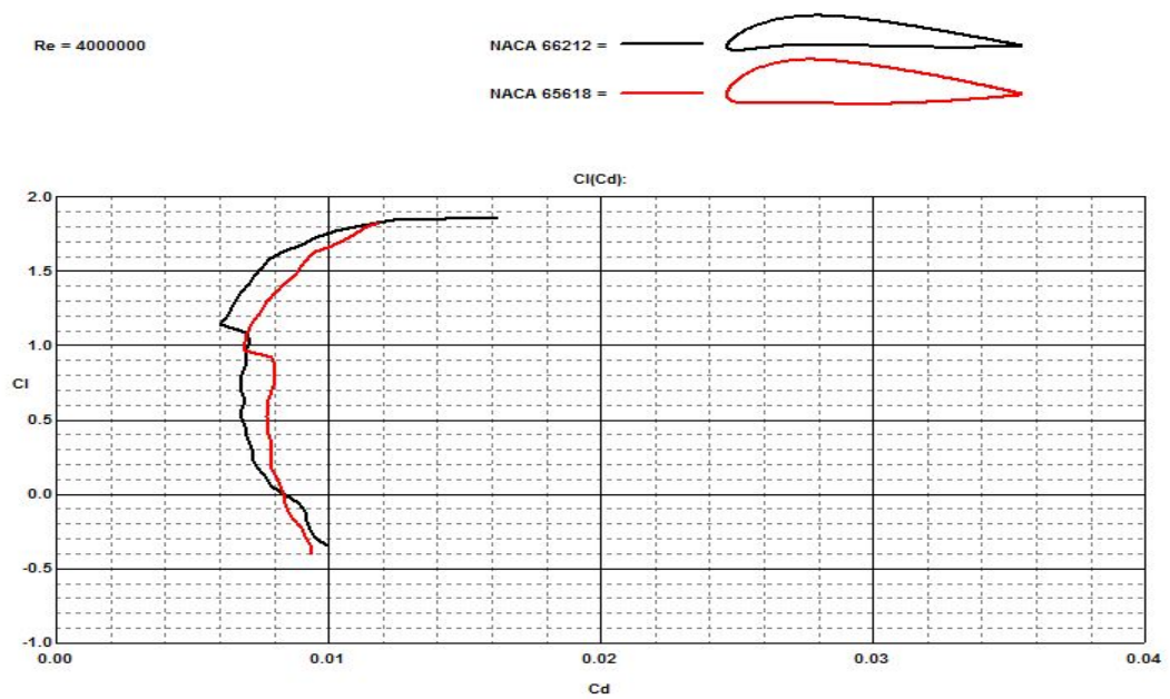
Figure 20. Comparison of the Drag Polars for the Naca 66212 and Naca 65618 Airfoils.
