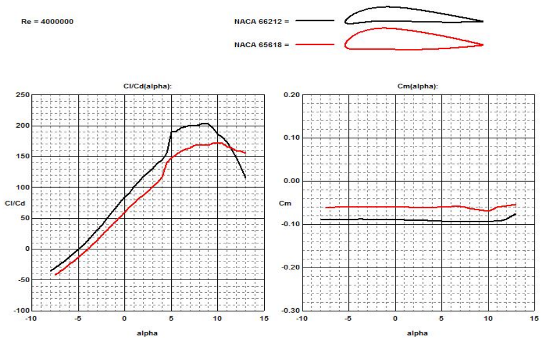
Figure 22. Comparison of the Lift-To-Drag Ratio and Pitching Moment of the Naca 66212 and Naca 65618 Airfoils.
