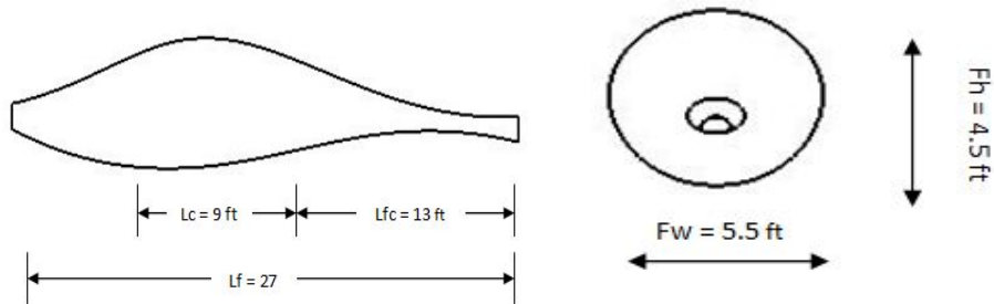
Figure 11. Fuselage Dimensions.
