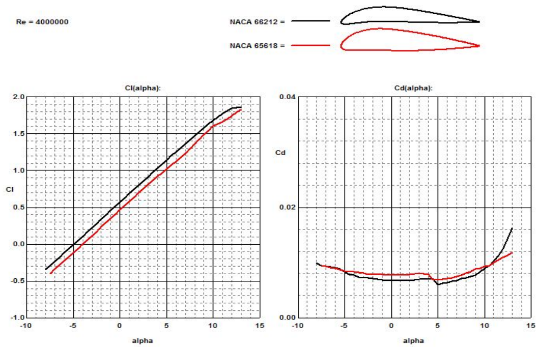
Figure 21. Comparison of the Lift and Drag Characteristics of the Naca 66212 and Naca 65618 Airfoils.
