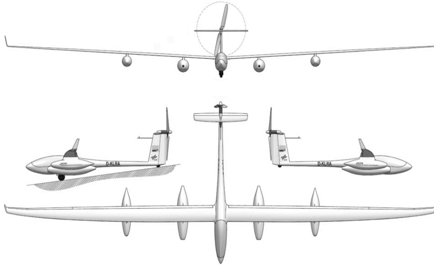
Figure 9. Antares H3 [9].
