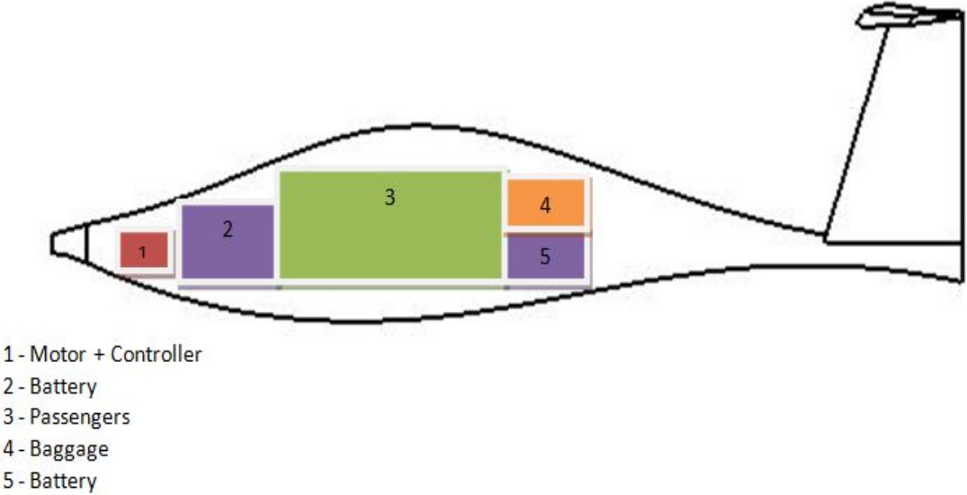
Figure 14. Location of Various Components for Estimating the CG Location
