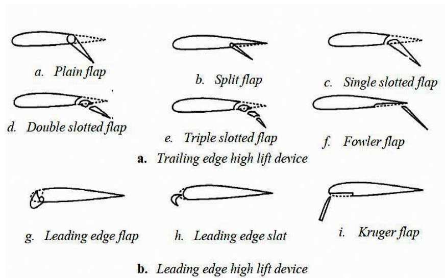
Figure 16. High Lift Devices [13].
