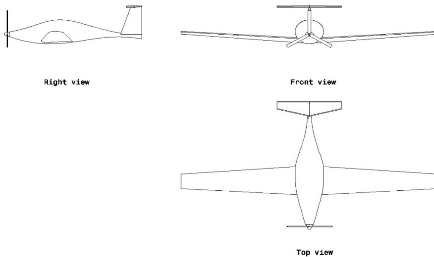
Figure 24. Electric Aircraft: Three View
