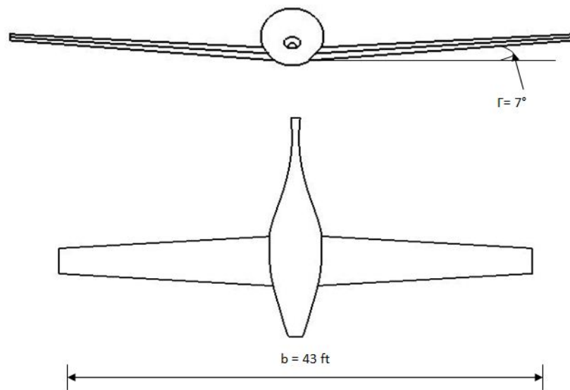
Figure 13. Wing specifications.
