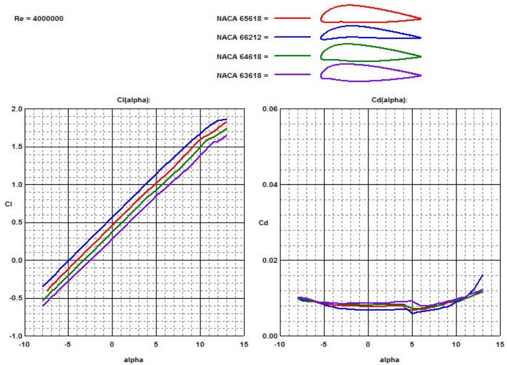
Figure 18. Lift and Drag Characteristics Comparison of Various Naca 6-Series Airfoils.
