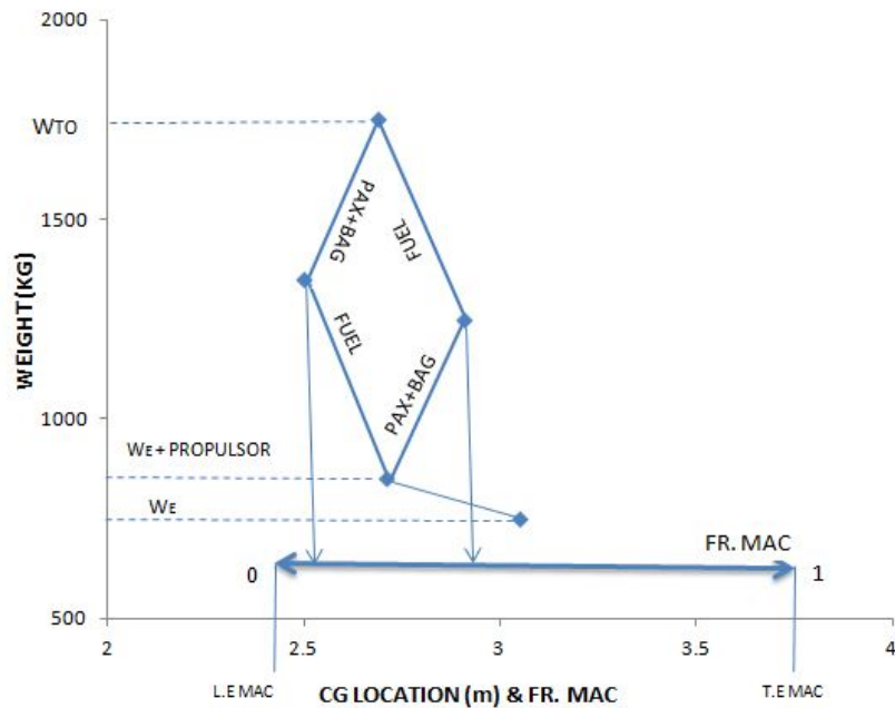
Figure 15. CG Excursion Diagram.
