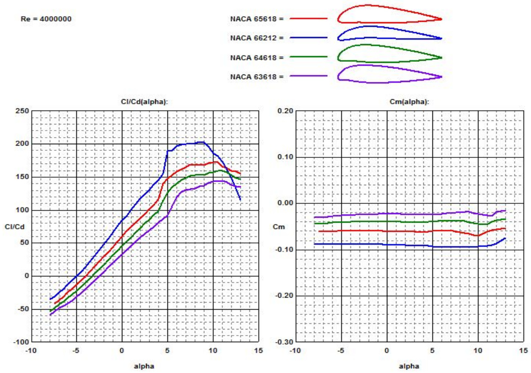
Figure 19. Lift-To-Drag Ratio and Pitching Moment Comparison of Various Naca 6-Series Airfoils
