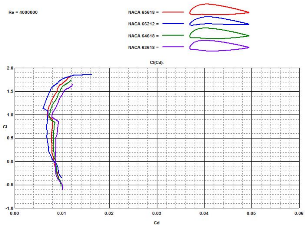
Figure 17. Drag Polar Comparison of Various Naca 6-Series Airfoils.
