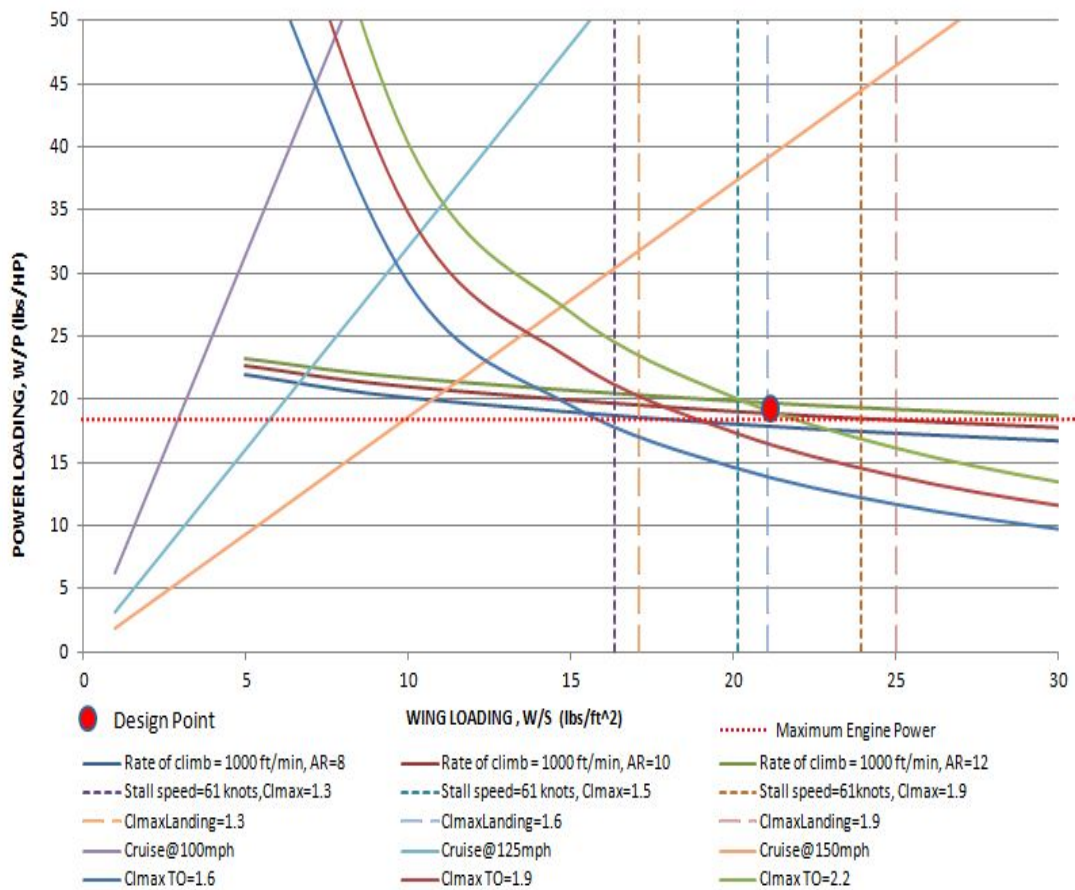
Figure 10. Performance Sizing Graph.
